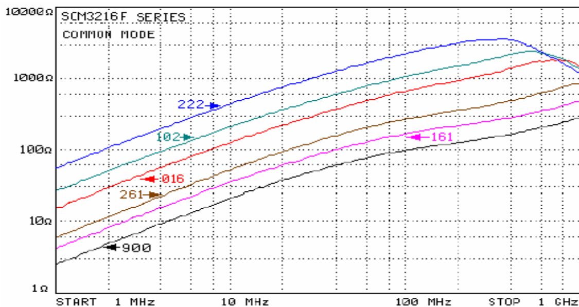
COMMON MODE
