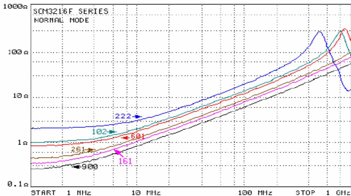
NORMAL MODE
