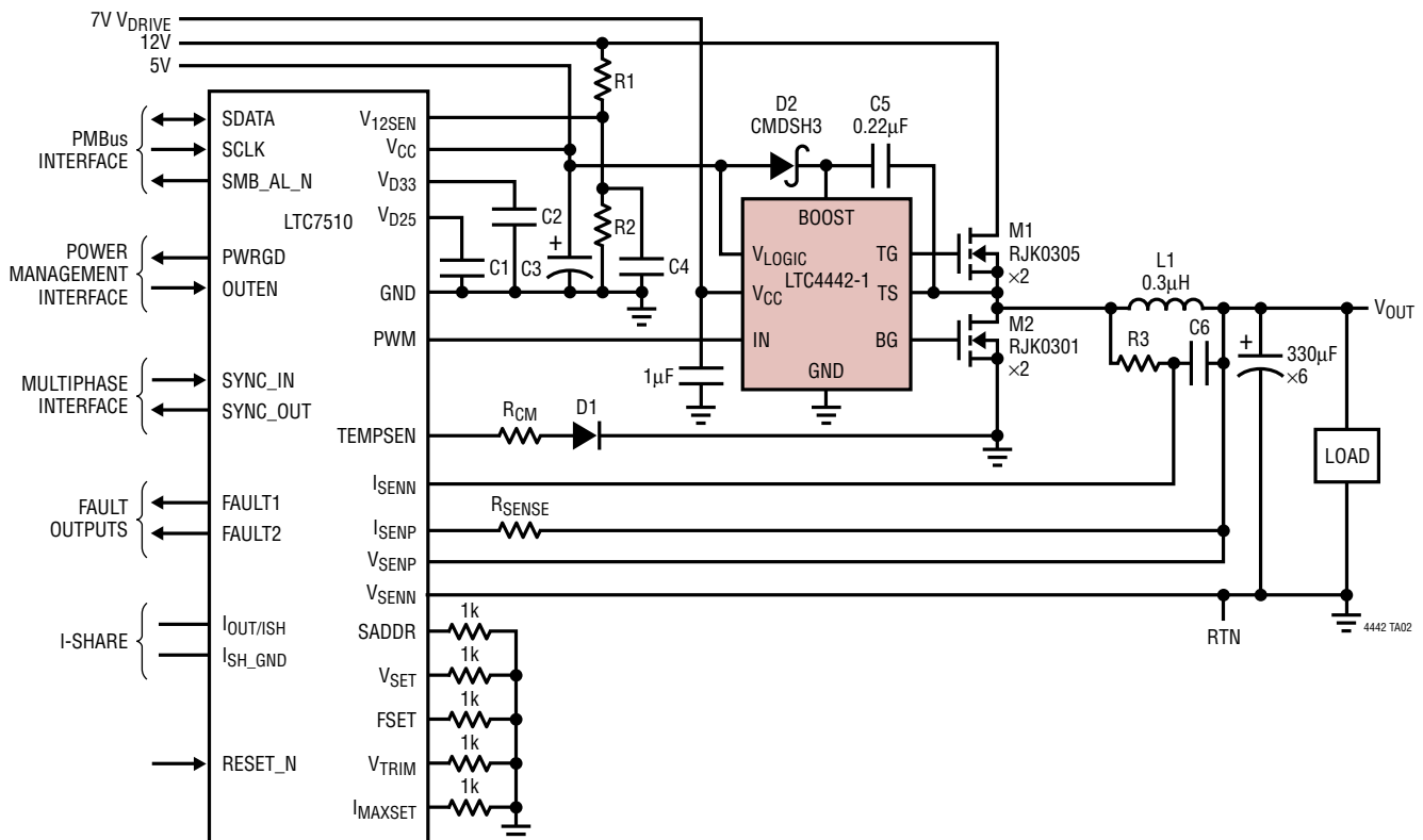
LTC7510/LTC4442-1 12V to 1.5V/30A Digital Step-Down DC/DC Converter with PMBus Serial Interface
