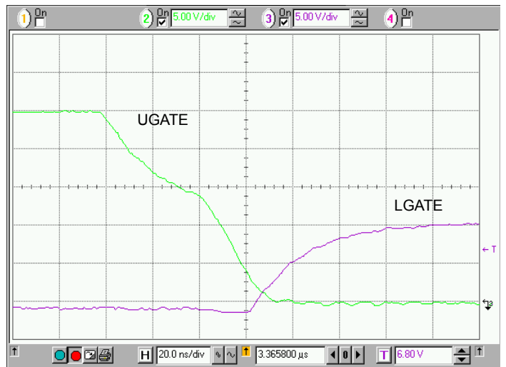
Time 20.0ns/Div.
