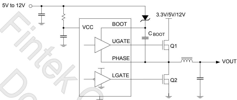
Fig 2. Power Supply Operation.
