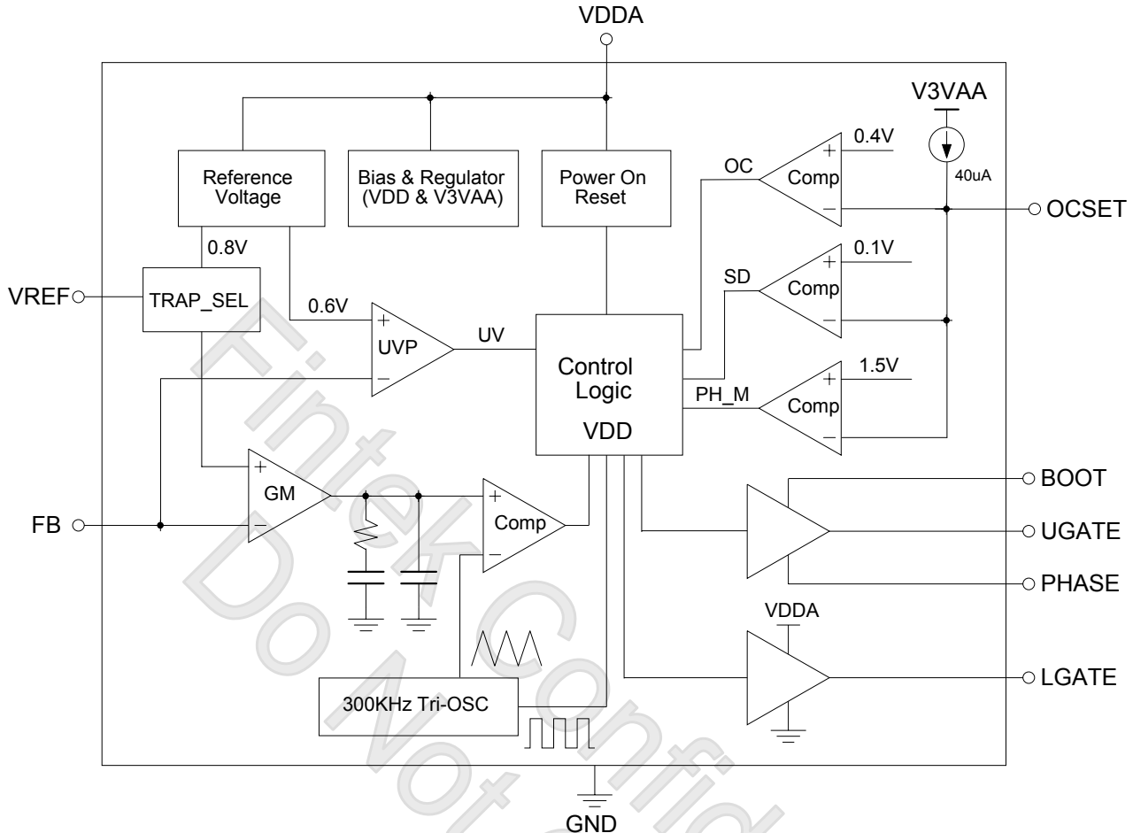
Figure 1: Block Diagram
