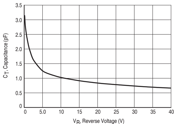
Figure 3. Typical Capacitance
