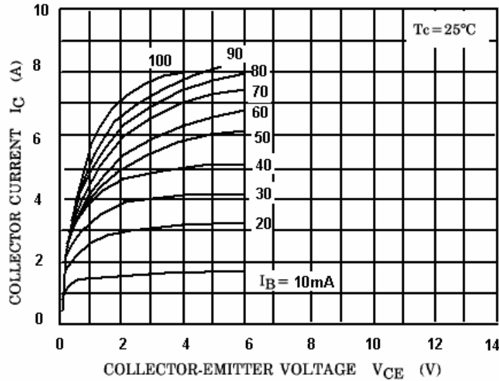
Fig.4 Static Characteristic
