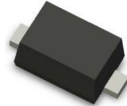
SOD-523F Band Indicates Cathode* Marking: 2B(521S)
