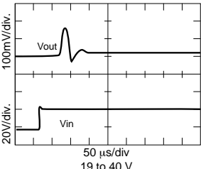
MFLHP2805S Step Line Response
