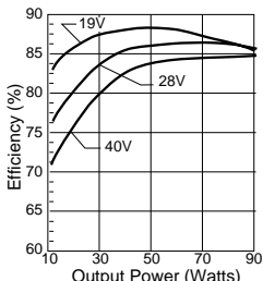
MFLHP2812S & MFLHP2812D Efficiency
