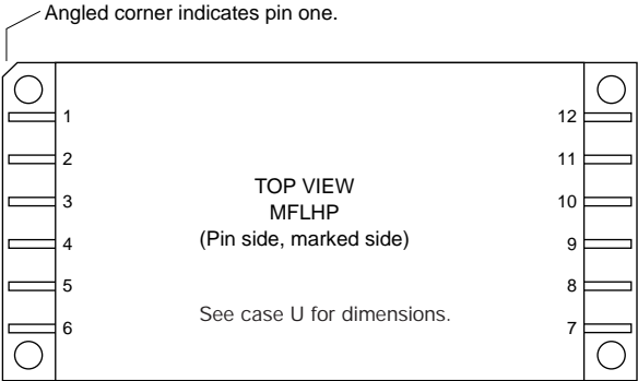
FIGURE 1: PIN OUT
