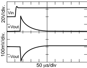
MFLHP2815D Step Line Response
