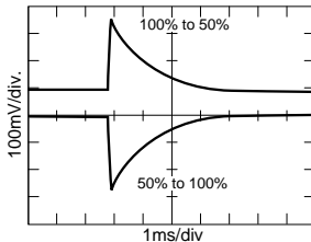
MFLHP2805S Step Load Response
