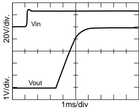
MFLHP2805S Turn On Response
