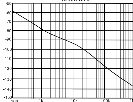
Phase Noise (dBc/Hz) 12500 MHz
