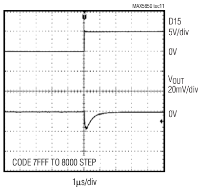
MAJOR-CARRY GLITCH (MAX5650)
