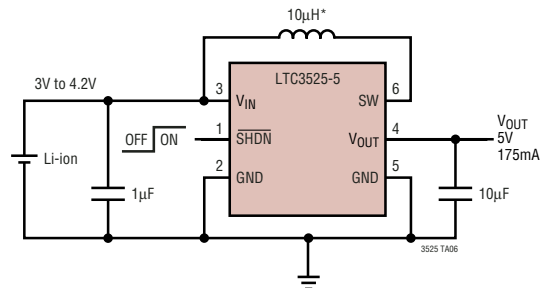
Li-Ion to 5V
