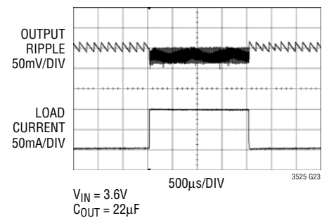
LTC3525-5 100mA Load Step Response
