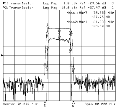
Horizontal: 8MHz/Div Vertical: 10dB/Div
