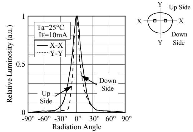
■ Directivity (NSPE800S)
