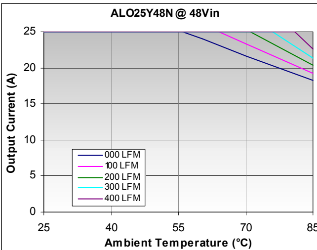
Figure 43. Output Current vs. Temperature for open frame version at V_{IN} = 48\text{Vdc} , T_A = 25^\circ\text{C} .
