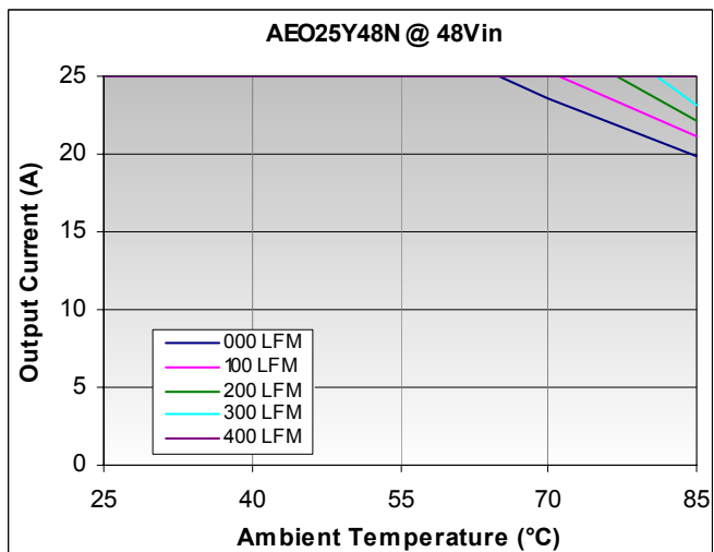
Figure 44. Output Current vs. Temperature for baseplate version at V_{IN} = 48\text{Vdc} , T_A = 25^\circ\text{C} .
