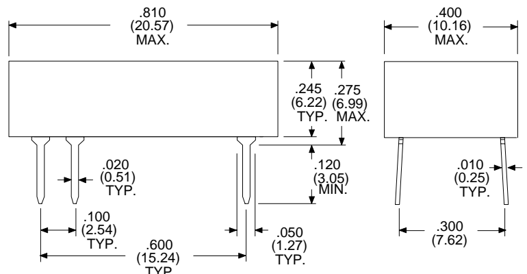
14-Pin Package with Unused Leads Removed Per Schematic
