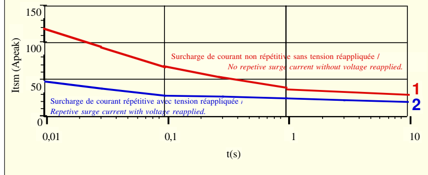
Fig 3 : Surcharge en courant : I_{t_{sm}}(A_{peak}) = f(t) pour modèle 12A ( I_{t_{sm}} = 120\text{A} ) / Surge current : I_{t_{sm}}(A_{peak}) = f(t) for 12A models with I_{t_{sm}} = 120\text{A}
