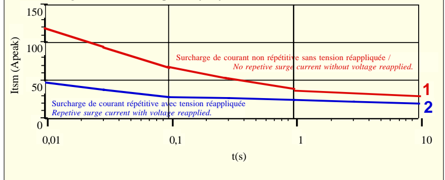
Fig.3 Surcharge de courant : I tsm (Apeak) = f(t) pour modèle 10A ( I tsm =120A) / Surge current : I tsm (Apeak) = f(t) for 10A models with I tsm =120A
