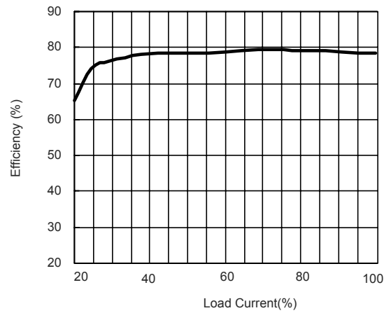
Efficiency vs Output Load ( Dual Output )
