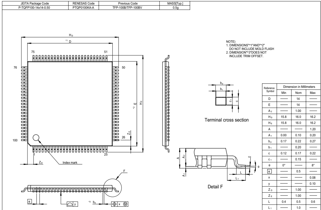
Figure C.1 TFP-100B Package Dimensions (H8S/2268 Group Only)
