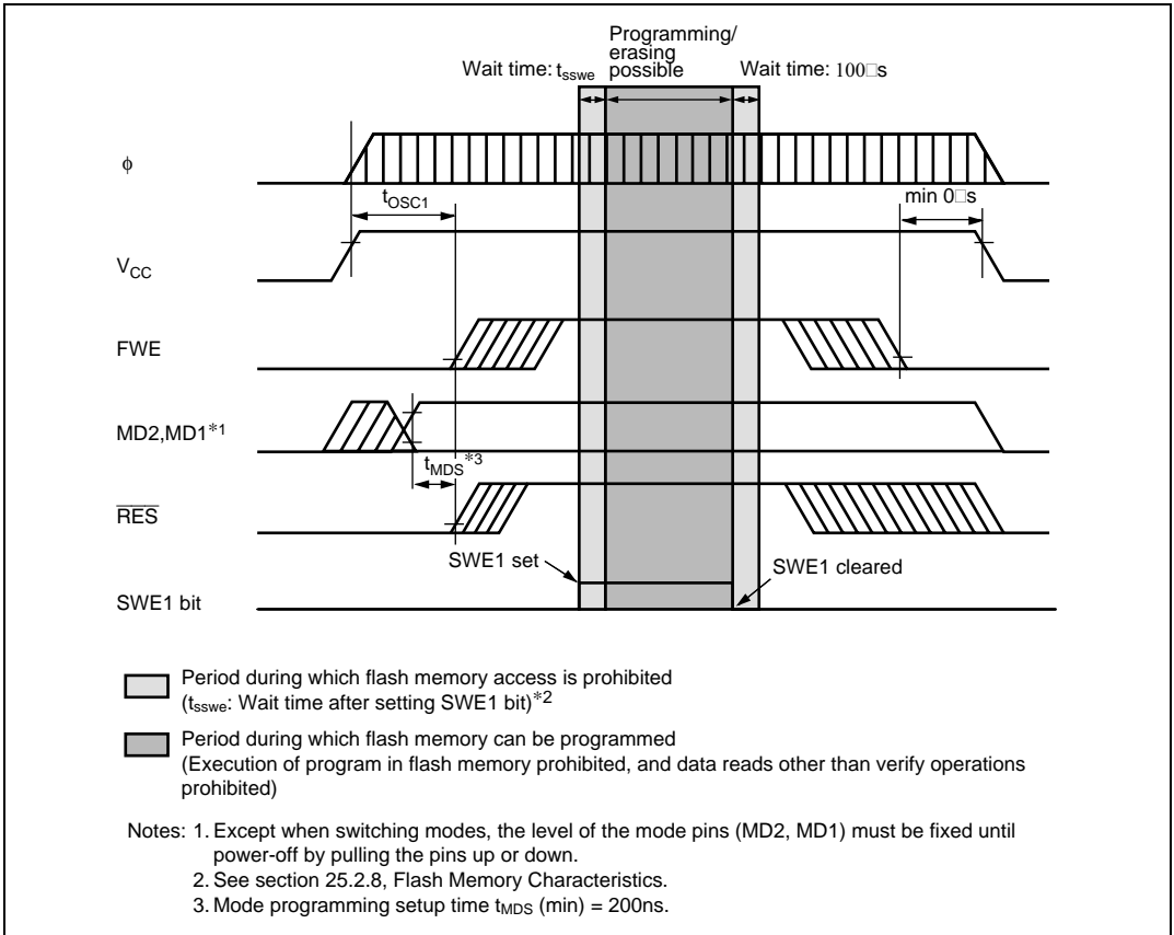
Figure 20.14 Power-On/Off Timing (User Program Mode)
