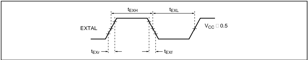
Figure 21.5 External Clock Input Timing
