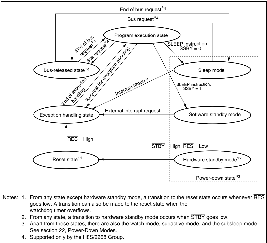
Figure 2.13 State Transitions
