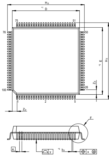
Figure C.3 FP-100B Package Dimensions
