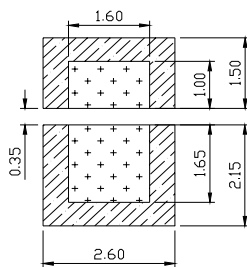
[ Normal Solder pad ]
