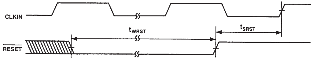
Figure 4. Reset
