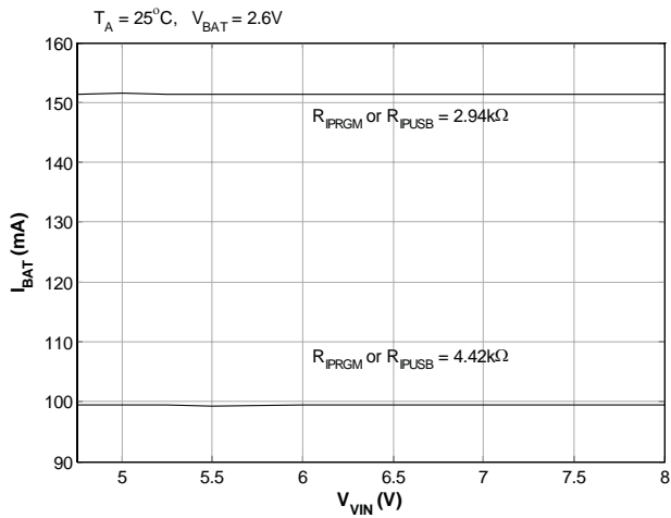
CC PQ Line Regulation
