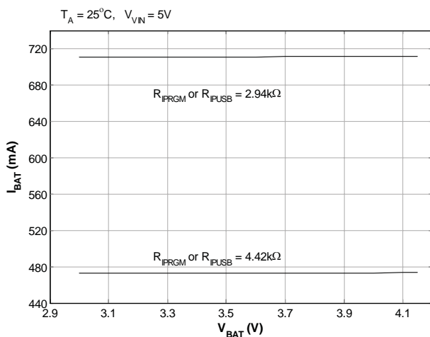
CC AD or USB High FQ V_{\text{BAT}} Regulation
