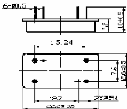
Package Outline
