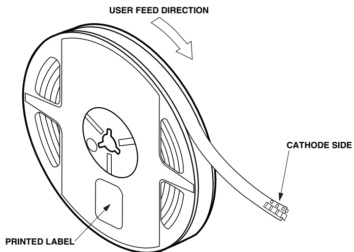
Figure 19. Reeling orientation.
