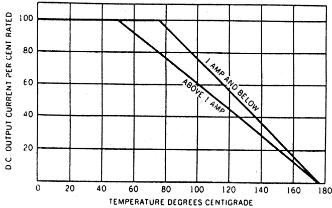
CURRENT VS. TEMPERATURE
