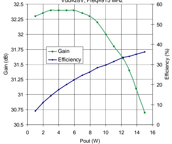
CW Gain, Efficiency vs Pout Vdd=28V, Freq=915 MHz
