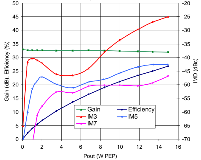
2 Tone Gain, Efficiency, Linearity vs Pout Vdd=28V, Freq=915 MHz, Delta F=1 MHz
