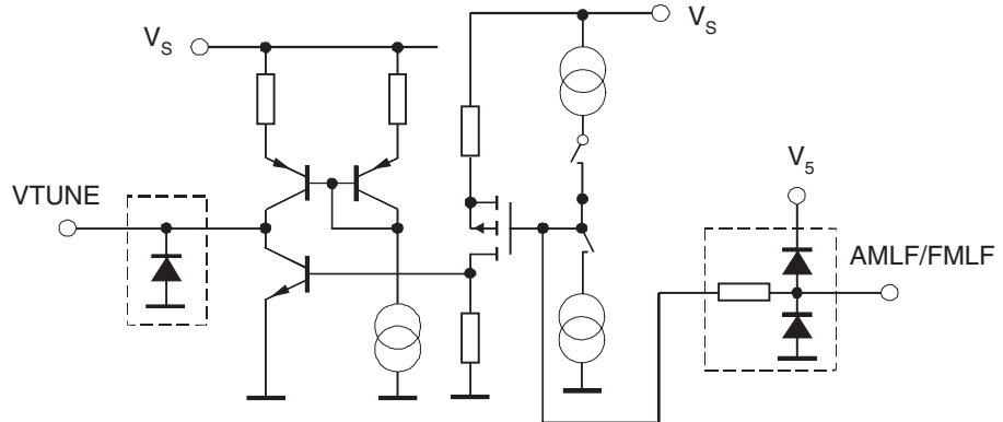
Figure 11-1. Internal Components at VTUNE, AMLF and FMLF
