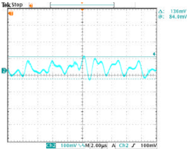
Figure 21. Output voltage Ripple & Noise at Vin=48v, Iout=0A, with 10uF tantalum cap. and 1uf ceramic cap. output capacitance load.
