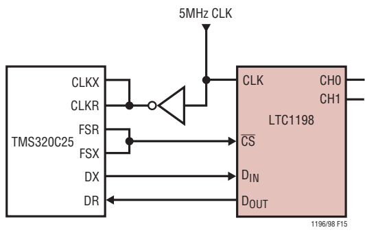
Figure 15. Interfacing the LTC1198 to the TMS320C25 DSP
