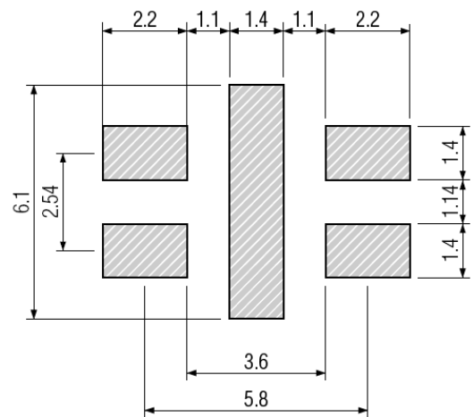
Figure 2) Land Pattern
