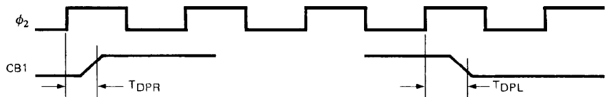
Figure 5k. Shift-in/out with Internal Clock Delay CD2 to CB1 Edge
