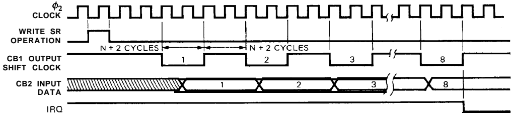
Figure 24-2 Shift Register Output Modes
