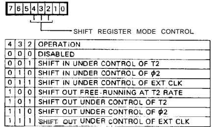
Figure 22. SR and ACR Control Bits
