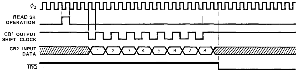
Figure 23-2 Shift Register Input Modes
