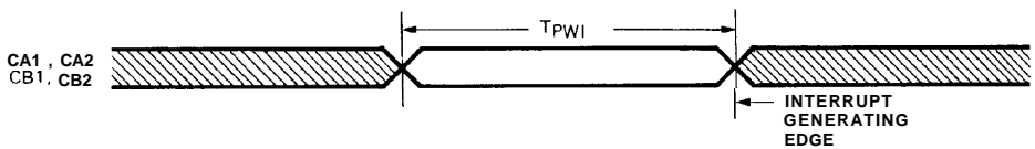
Figure 5j. Setup Time to Trigger Edge
