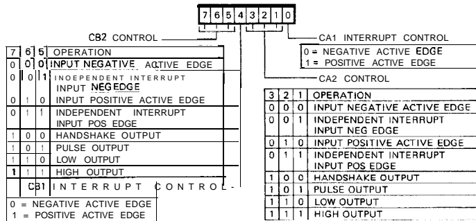
Figure 14. CA1, CA2, CB1, CB2 Control
