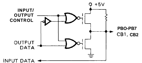
Figure 8. Peripheral B Port Output Circuit
