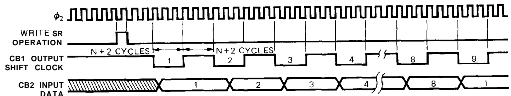
Figure 24-1 Shift Register Output Modes
