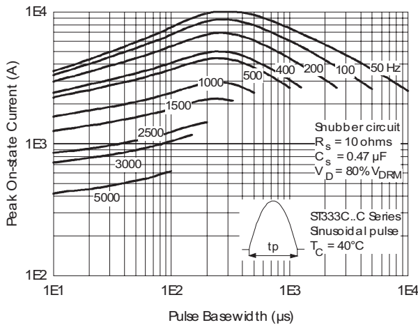
Fig. 13 - Frequency Characteristics
