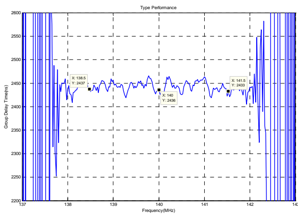
Group Delay Variation( f_0 \pm 1.5\text{MHz} )
