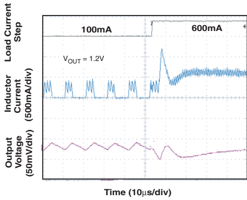
Figure 11. Load Transient Response
