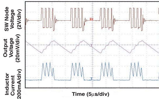
Figure 10. Power-Save Mode
