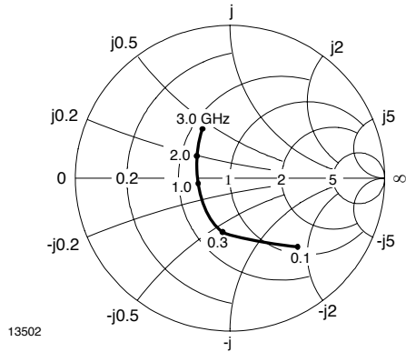
Figure 6. Input Reflection Coefficient
