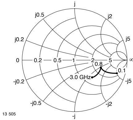
Figure 9. Output Reflection Coefficient
