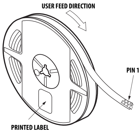
Figure 15. Reeling Orientation
