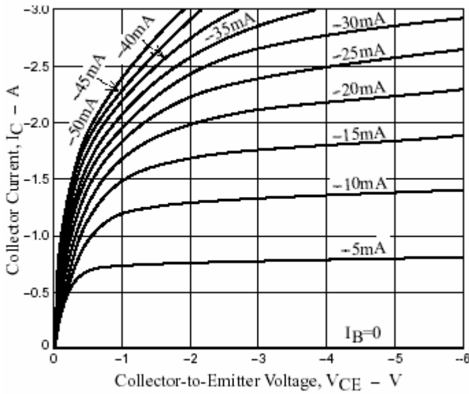
Fig.3 Static Characteristic
