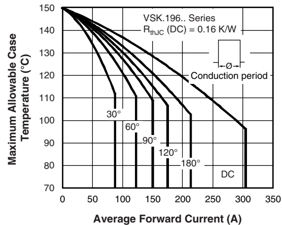
Fig. 11 - Current Ratings Characteristics
