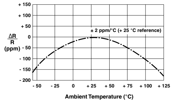
FIGURE 4 - TYPICAL TCR CURVE
