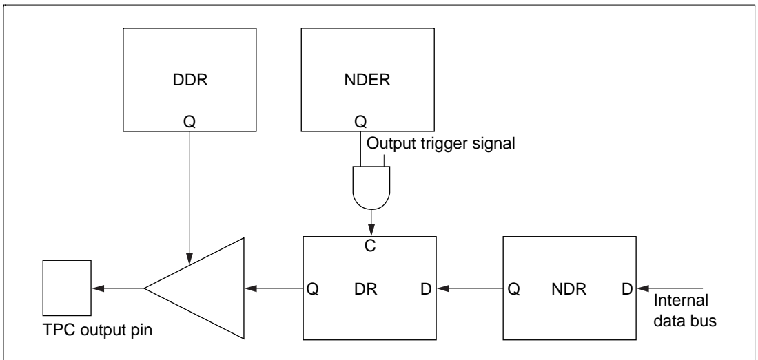
Figure 12.2 TPC Output Operation
