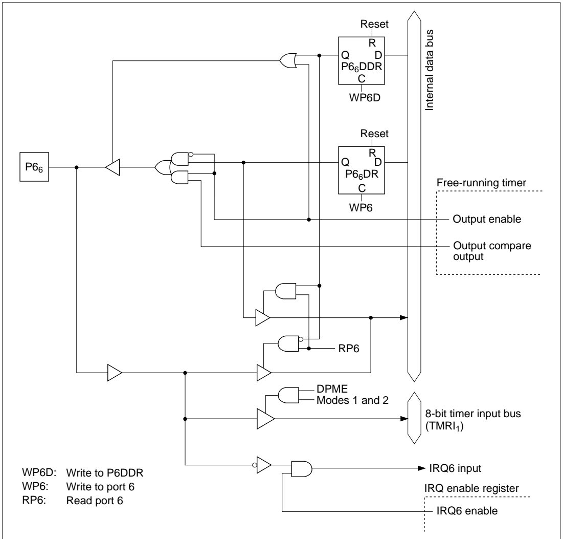
Figure C.6 (e) Port 6 Block Diagram (Pin P6 6 )
