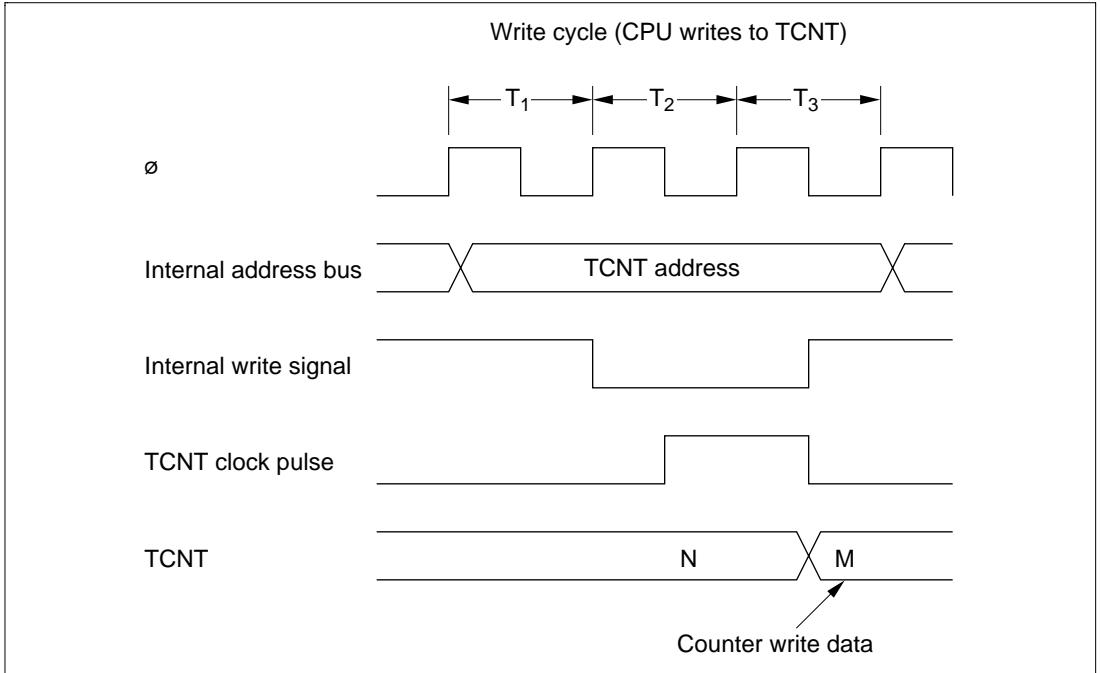
Figure 13.6 TCNT Write-Increment Contention
