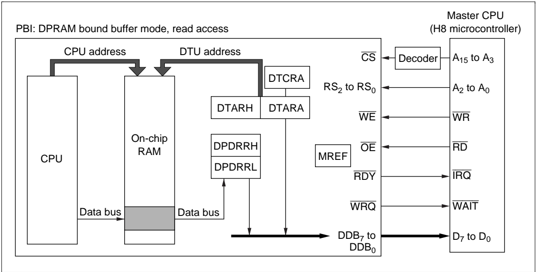
Figure 5.16 Read Access in DPRAM Bound Buffer Mode
