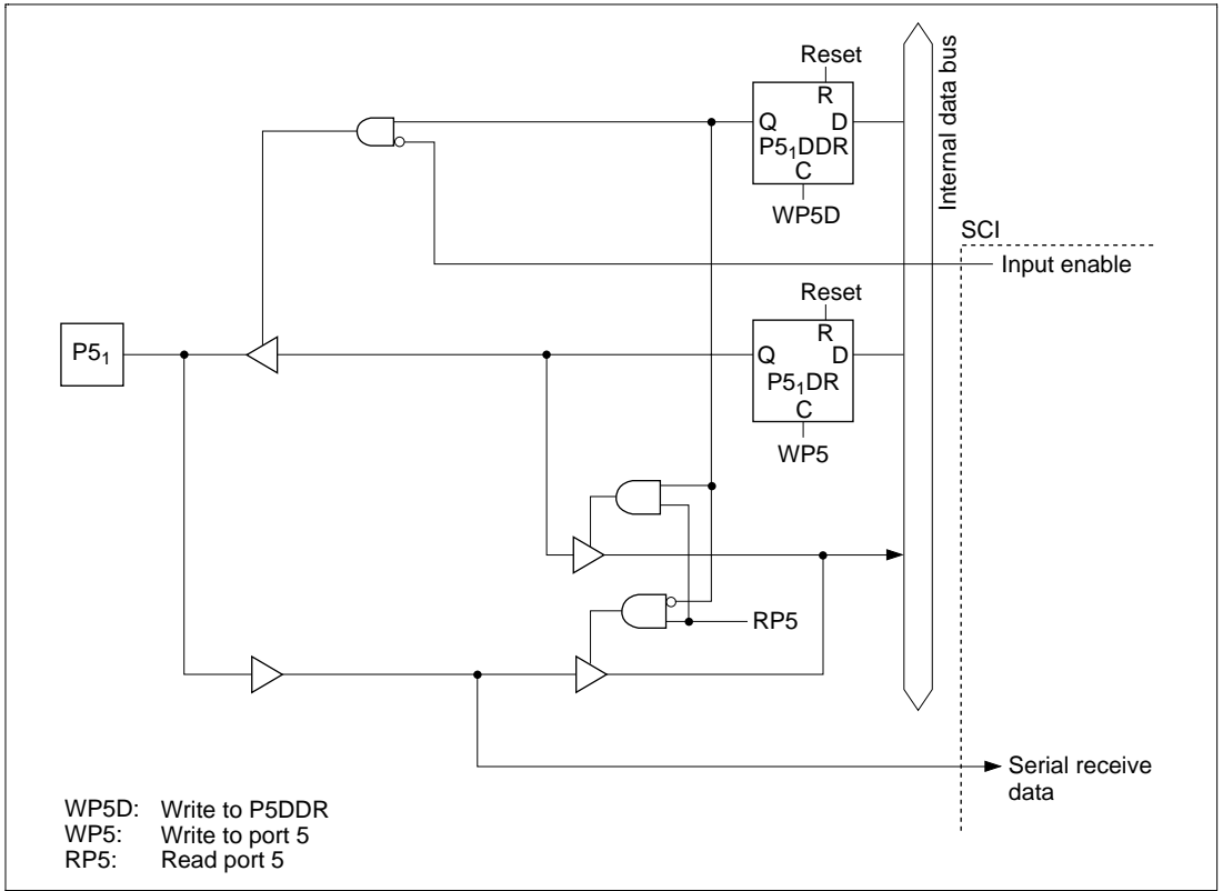
Figure C.5 (b) Port 5 Block Diagram (Pin P5 1 )
