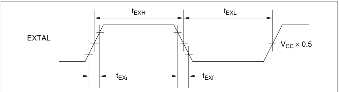
Figure 7.6 External Clock Input Timing
