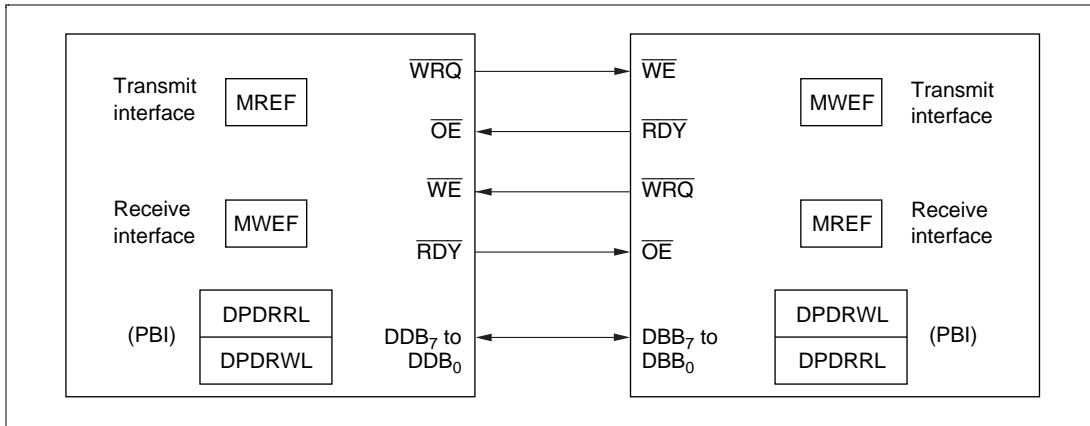
Figure 5.24 Interconnections for Handshake Mode (Example)
