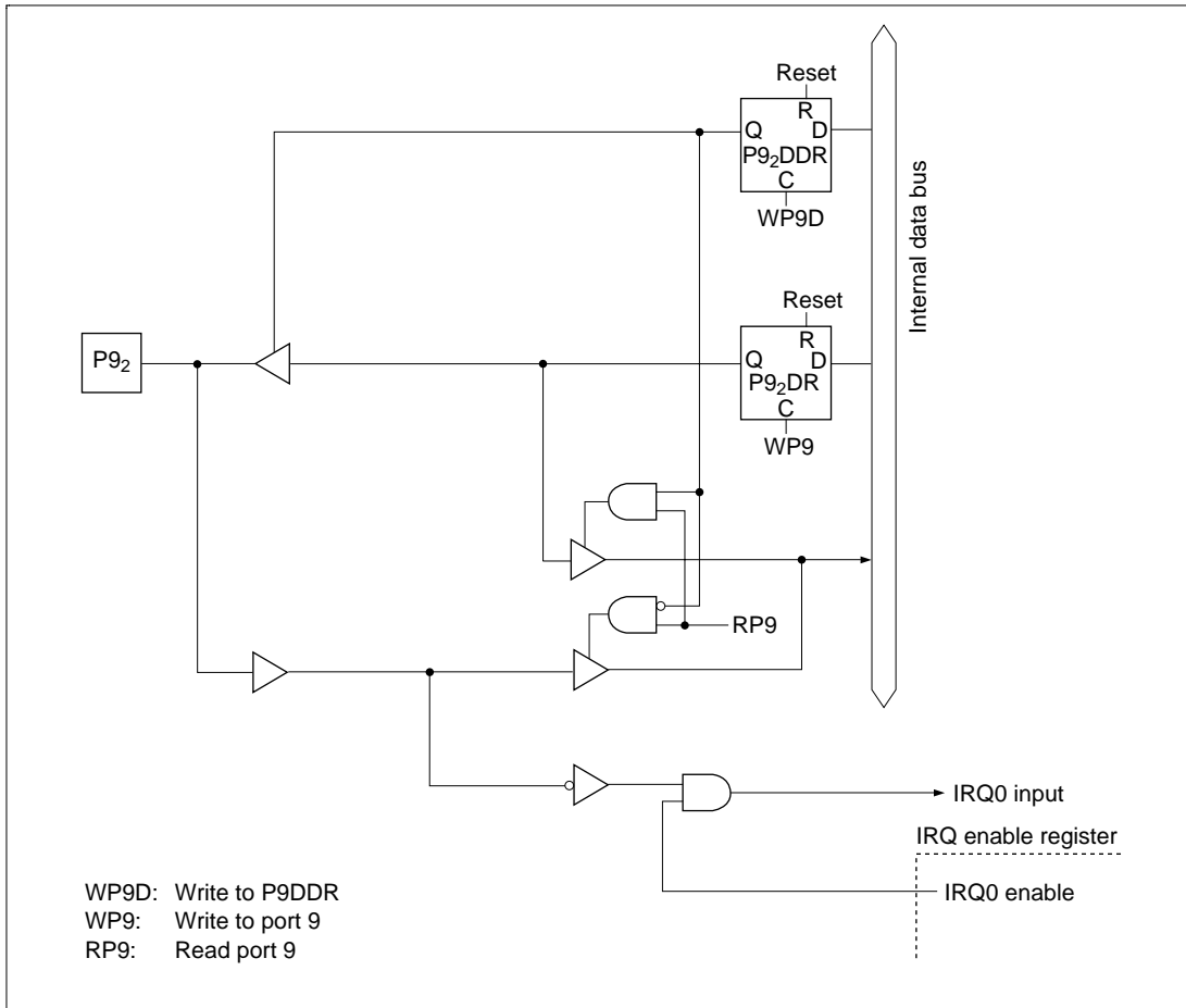
Figure C.9 (c) Port 9 Block Diagram (Pin P9 2 )
