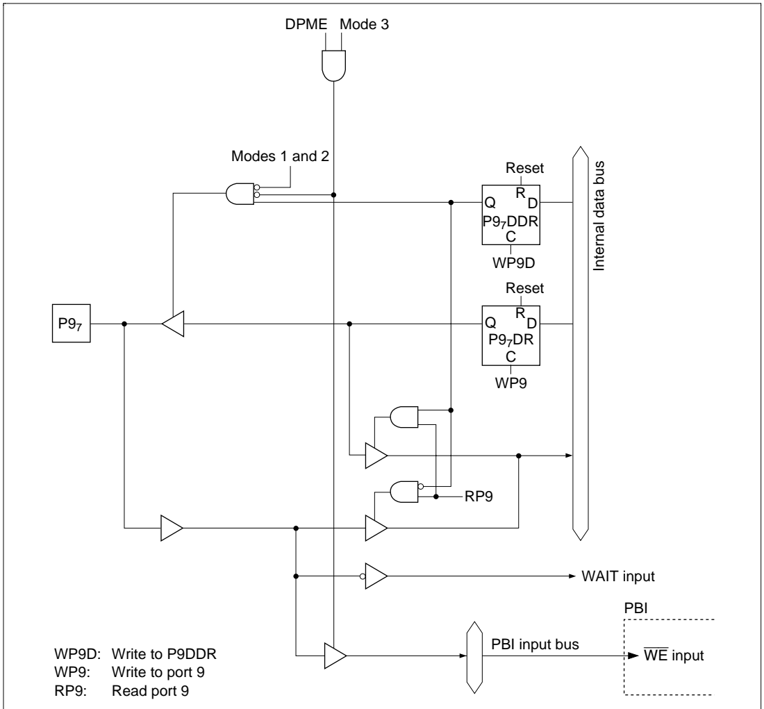
Figure C.9 (g) Port 9 Block Diagram (Pin P9 7 )
