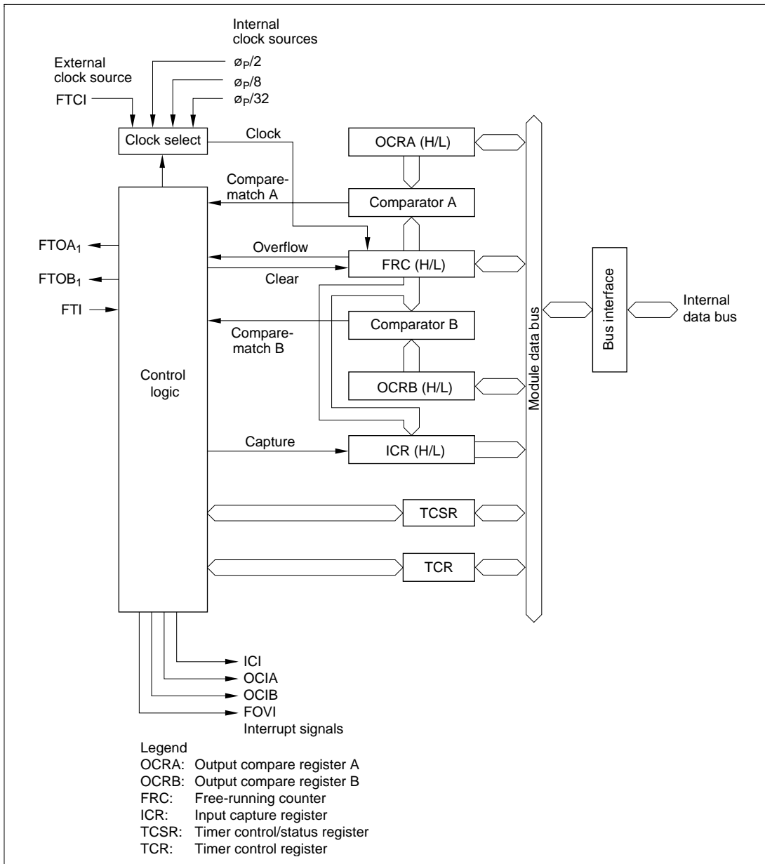
Figure 10.1 Block Diagram of 16-Bit Free-Running Timer 1
