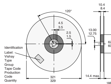
Figure 10. Reel dimensions - GS18
