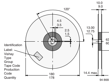
Figure 9. Reel dimensions - GS08
