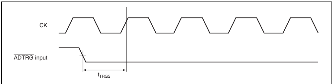
Figure 21.15 External Trigger Input Timing
