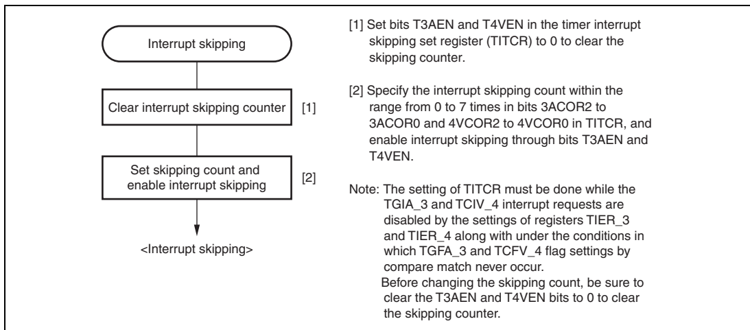
Figure 9.67 Example of Interrupt Skipping Operation Setting Procedure
