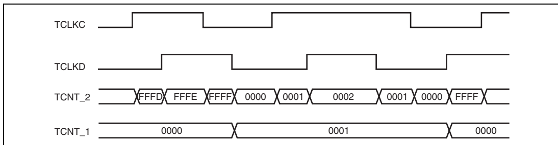
Figure 9.21 Cascaded Operation Example (a)
