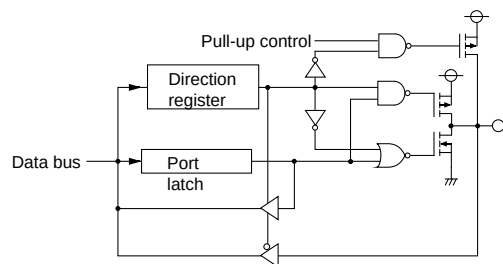
(11) Ports P30–P35
