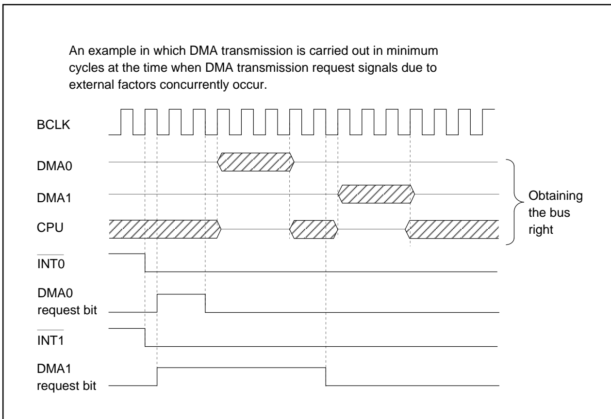
Fig.EC-6 An example of DMA transfer effected by external factors
