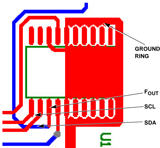
FIGURE 21. SUGGESTED LAYOUT FOR THE ISL12022M
