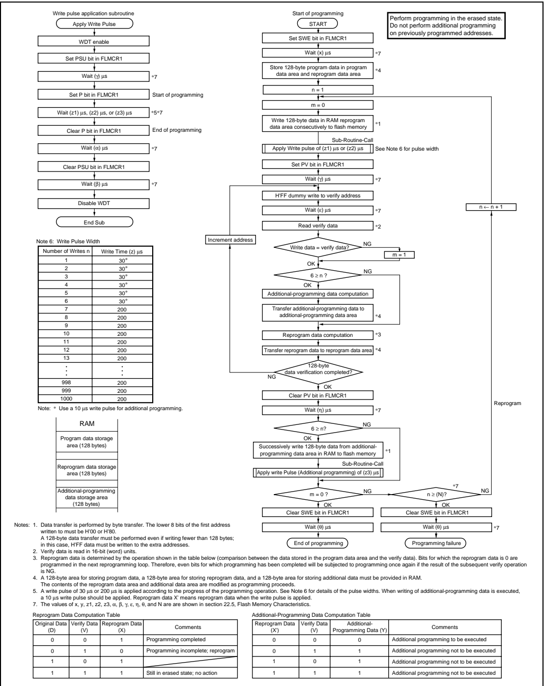
Figure 16.9 Program/Program-Verify Flowchart
