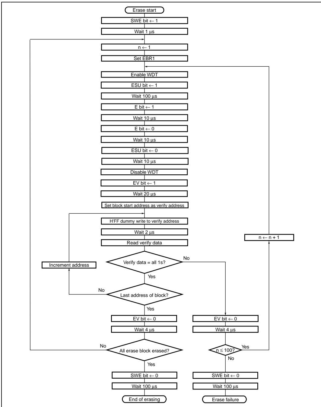
Figure 17.8 Erase/Eraser-Verify Flowchart
