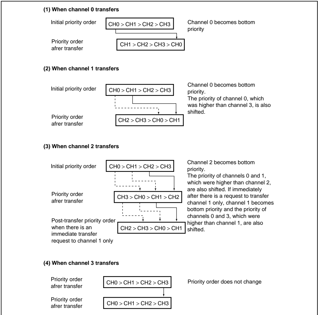
Figure 9.3 Round-Robin Mode
