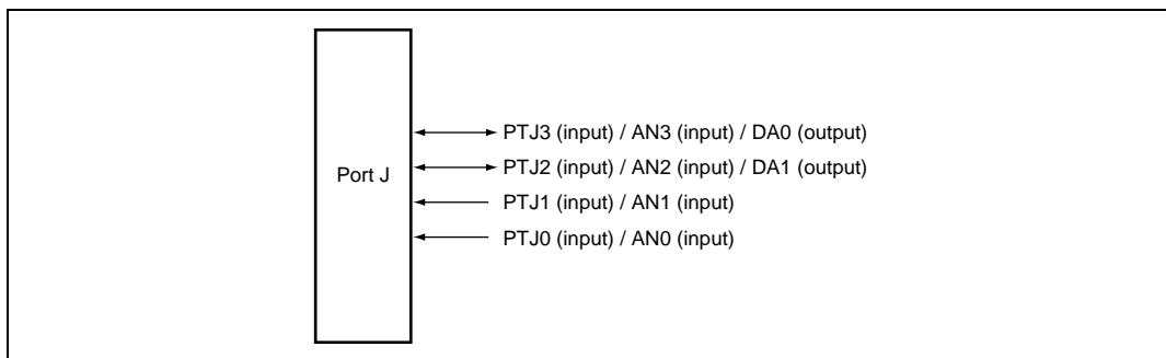
Figure 18.9 Port J
