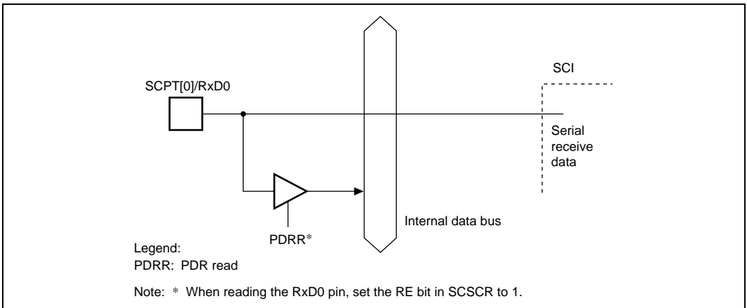
Figure 14.4 SCPT[0]/RxD0 Pin
