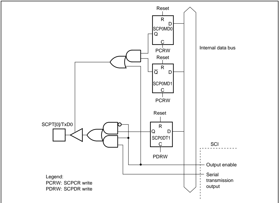
Figure 14.3 SCPT[0]/TxD0 Pin
