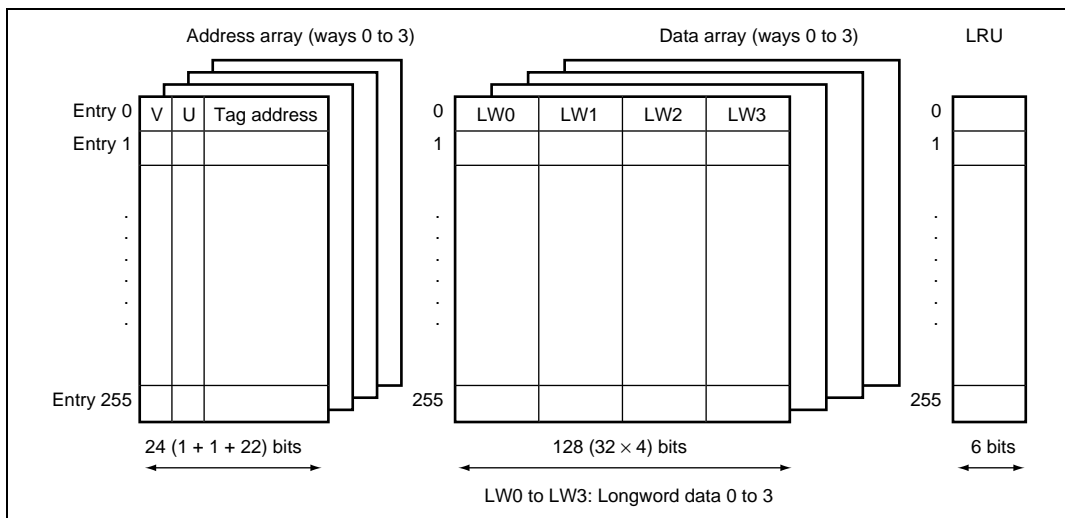
Figure 5.1 Cache Structure
