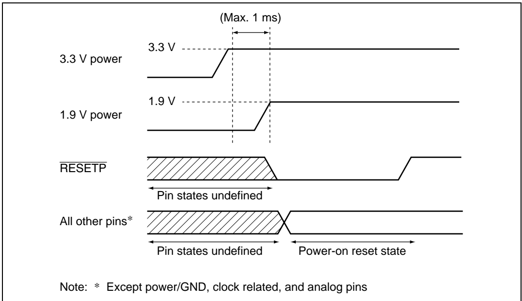
Power-On Sequence
