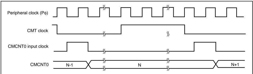
Figure 9.28 Count Timing
