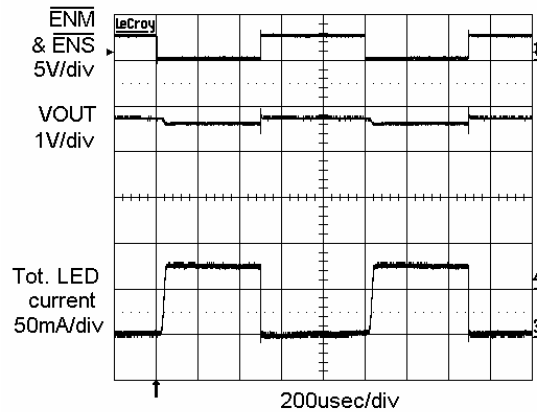
PWM Dimming at 1kHz on \overline{ENM} and \overline{ENS}
