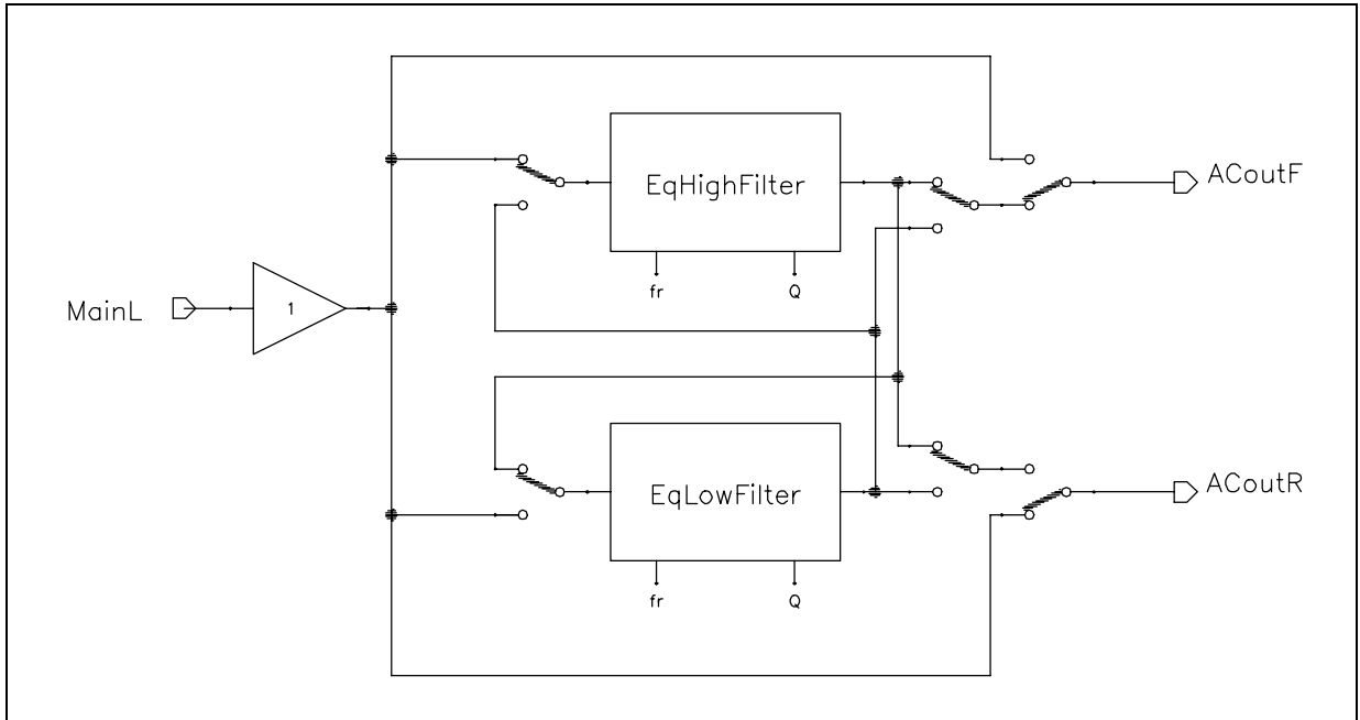
Figure 17. Equalizer Configuration
