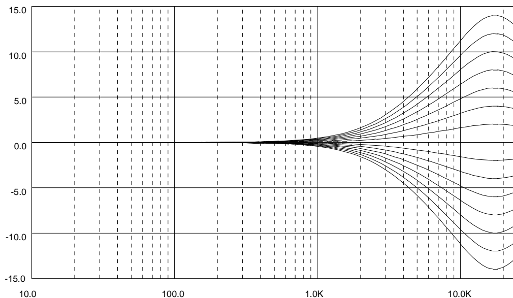
Figure 15. Treble Control @ f_C = 17.5\text{kHz}
