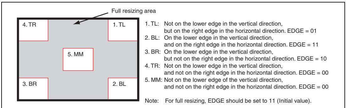
Figure 28.38 Examples of Partial Resizing Areas
