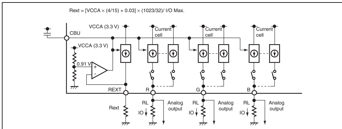
Figure 28.59 Current Cells and Analog Outputs
