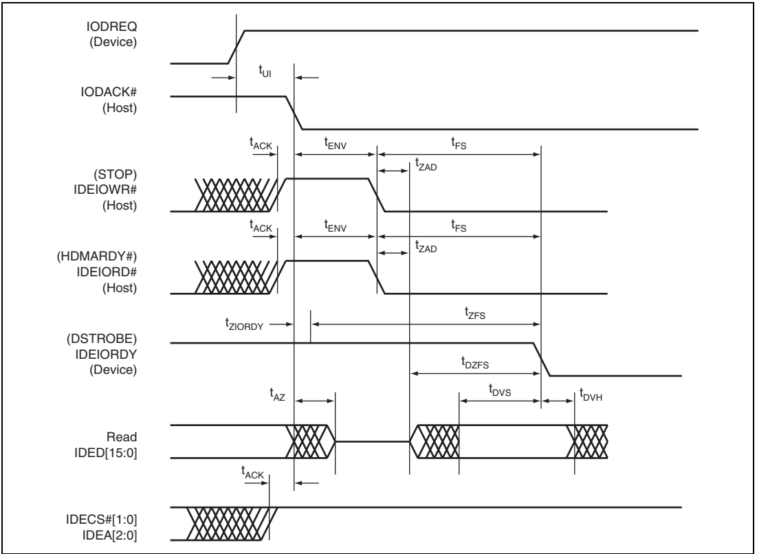
Figure 36.65 Initiating Ultra DMA Data-In Burst
