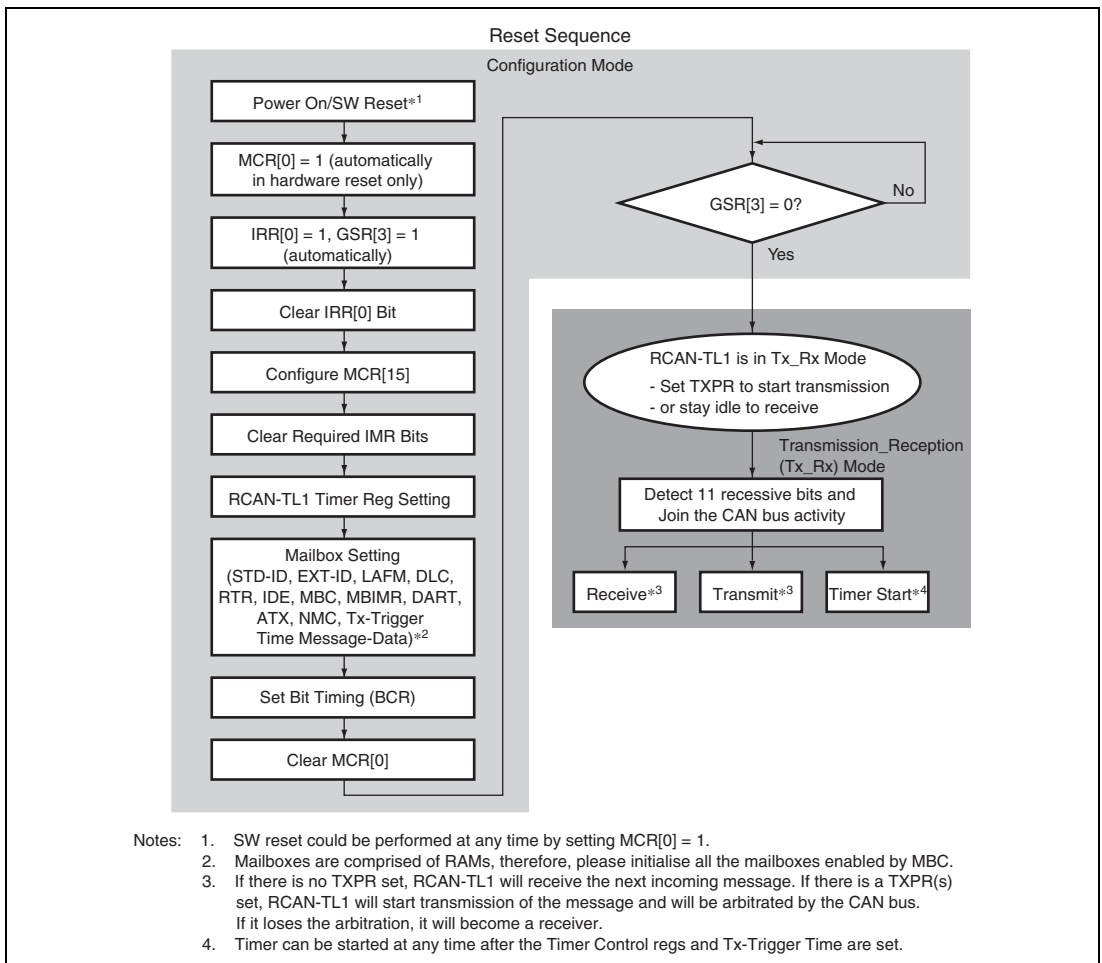
Figure 20.14 Reset Sequence
