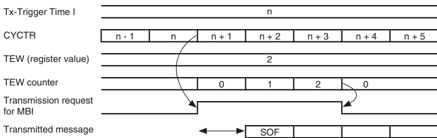
Figure 20.23 Timing Diagram of Timer
