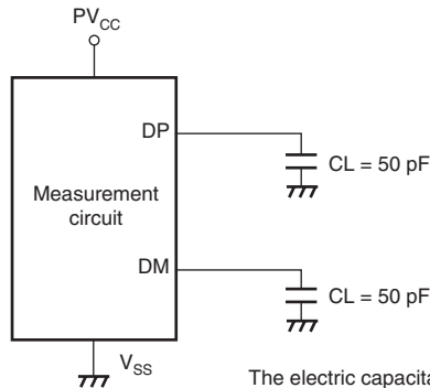
Figure 36.57 Measurement Circuit (Full-Speed)
