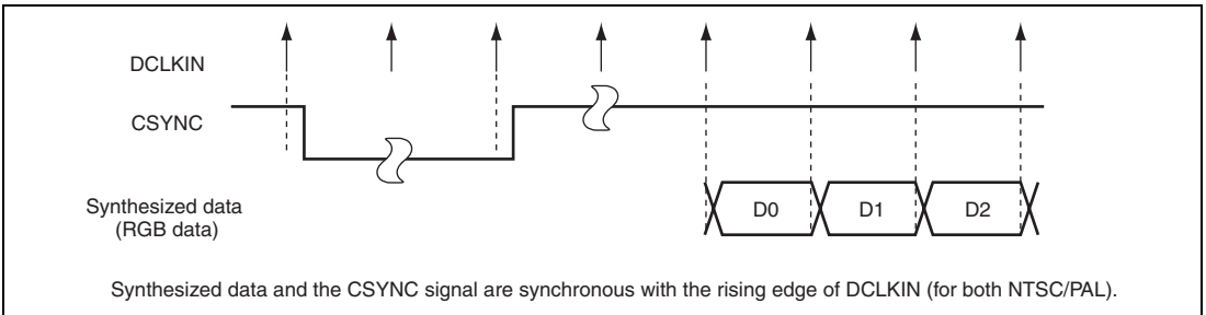
Figure 28.14 2DG Output Signals and DCLKIN
