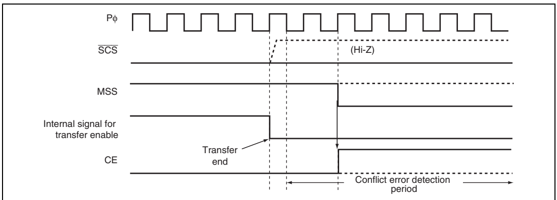
Figure 17.11 Conflict Error Detection Timing (After Transfer End)
