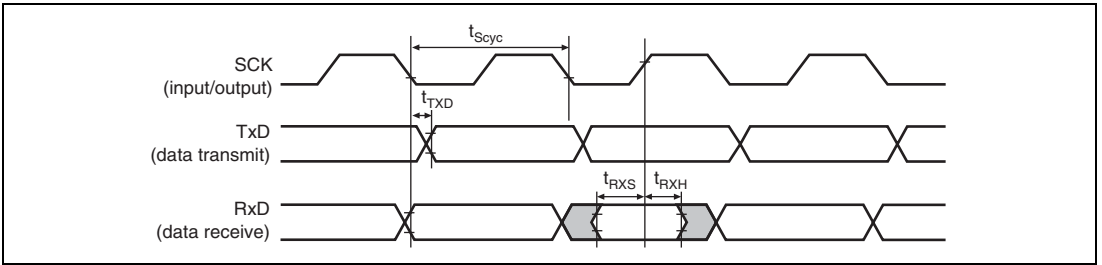
Figure 36.30 SCIF Input/Output Timing in Clocked Synchronous Mode
