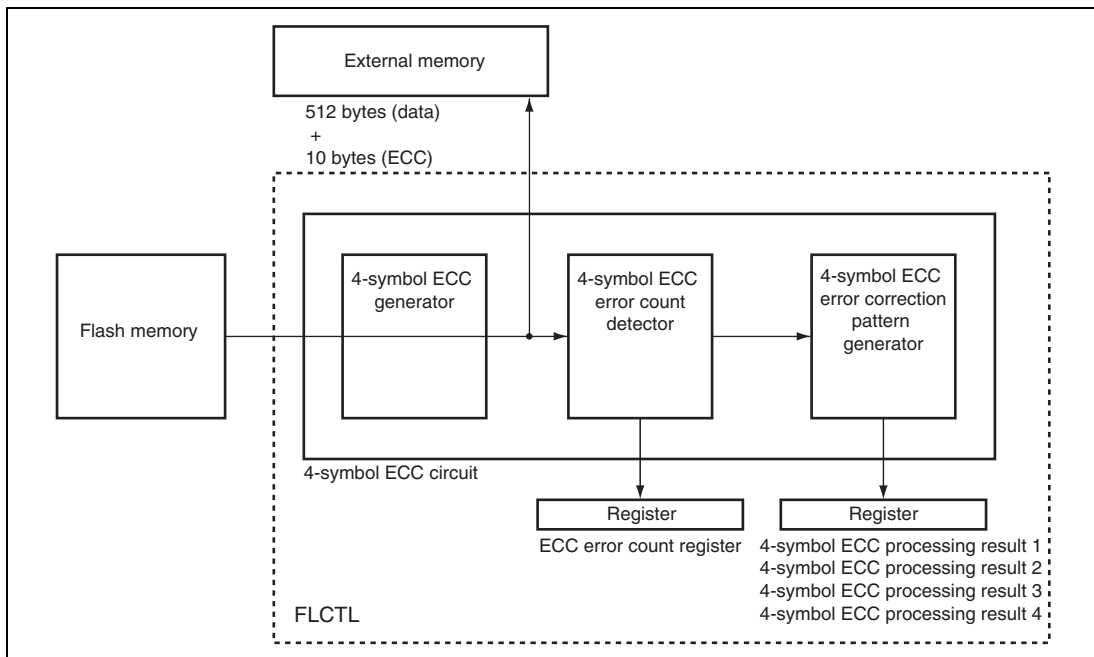
Figure 24.17 4-Symbol ECC Circuit
