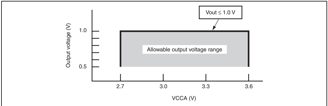
Figure 28.60 Allowable Analog Output Voltage Range
