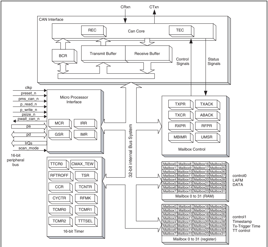
Figure 20.1 RCAN-TL1 architecture
