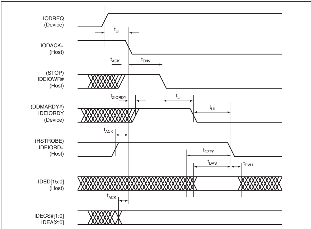
Figure 36.70 Initiating Ultra DMA Data-Out Burst
