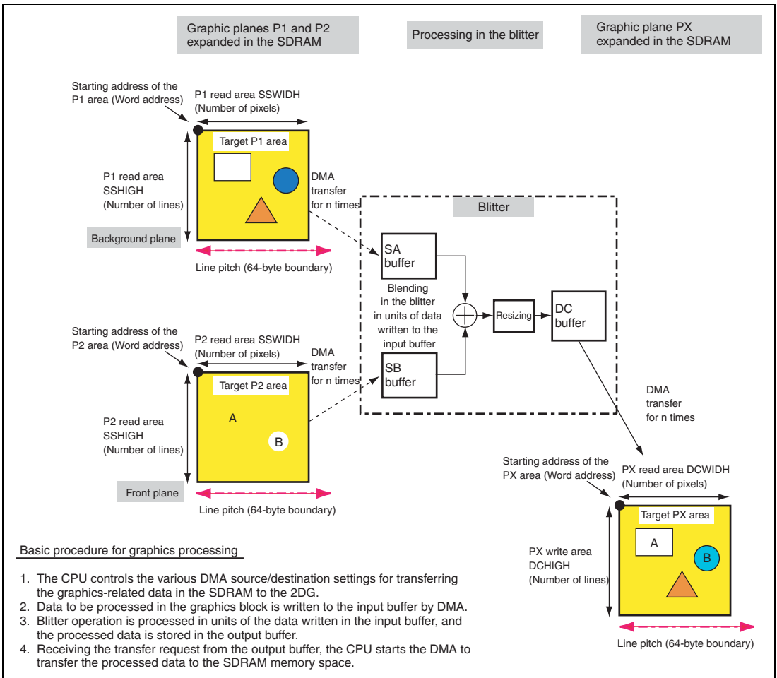
Figure 28.20 Summary of Blitter Operations
