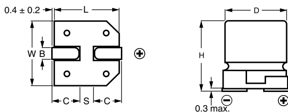
Fig.2 Dimensional outline
